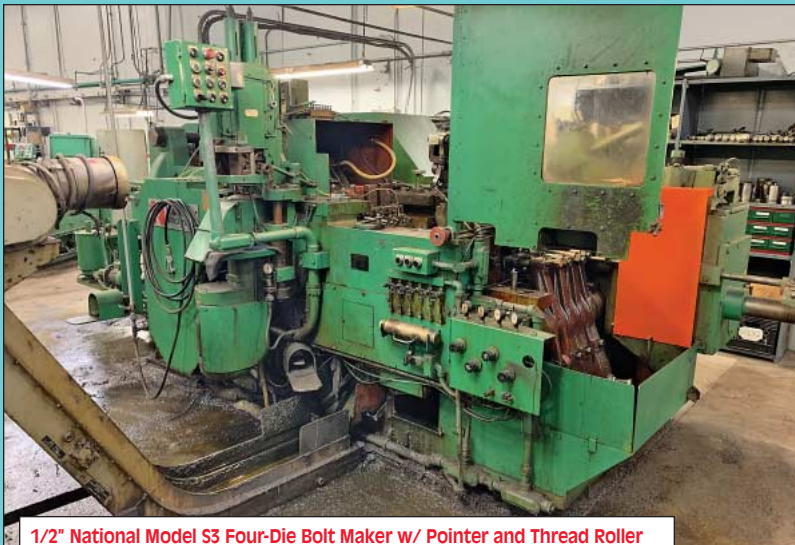
1/2" National Model S3 Four-Die Bolt Maker w/ Pointer and Thread Roller
